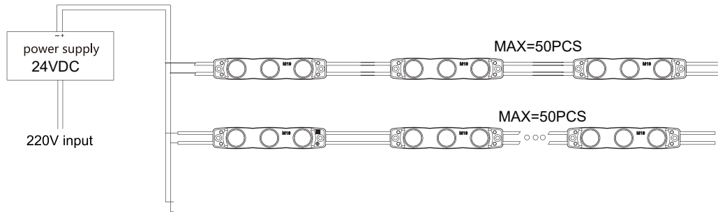
Connection Diagram
