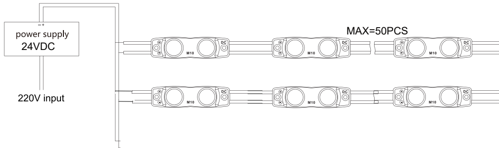
Connection Diagram
