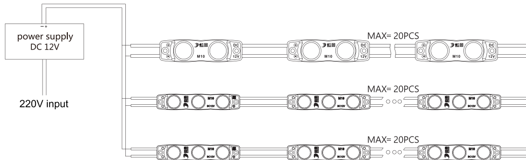
Connection Diagram
