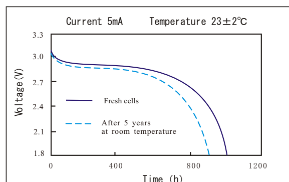
Storage Characteristics
