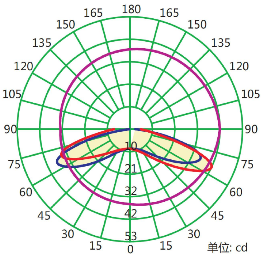
Beam angle 168°
